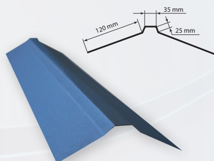
GAŚSIORY DO BLACHODACHÓWKI
